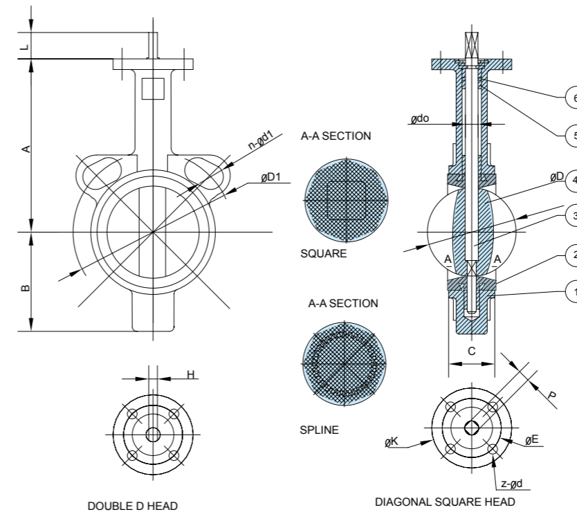
Wafer Butterfly Valve ( Two Holes With Tongue - And - Groove Seat )
