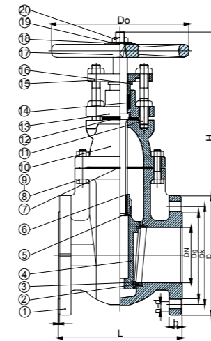
Non-Rising Stem Solid Wedge Gate Valve (BS5150)
