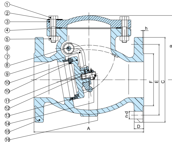
Swing Check Valve (BS5153)
