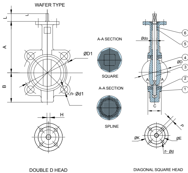
Wafer Butterfly Valve ( Four Holes With Tongue - And - Groove Seat )
