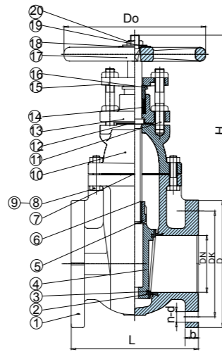
Non-Rising Stem Solid Wedge Gate Valve (ANSI B16.10)
